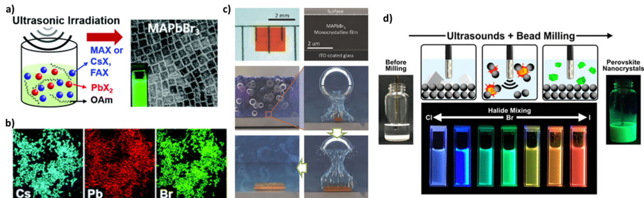
Fig. 13 (a) Ultrasound-induced synthesis of APbX 3 perovskite nanocrystals with a wide range of compositions, where A = CH 3 NH 3 , Cs, or HN=CHNH 3 (formamidinium), and X = Cl, Br, or I. (b) EDX maps showing homogeneous distributions of Cs, Pb, and Br in CsPbBr 3 NCs. Adapted with permission from ref. 186. (c) Optical image of the monocrystalline film (left). Cross-sectional SEM image of a freshly cut monocrystalline film (right). Illustrations of the CTAC mechanism on a microscopic scale. Adapted with permission from ref. 187. (d) Schematic illustration of the ultrasound-assisted bead milling (top) and photograph under a UV lamp of the colloidal halide-mixed perovskite nanocrystals. Adapted with permission from ref. 189.
