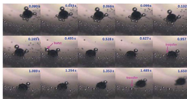
Fig. 2 Time lapse images of Au-GCB-Pt were extracted from Movie S3† (1.6 \times magnification objective lens). 6 mL fuel solution containing 0.526% \text{H}_2\text{O}_2 , 0.021 \text{g L}^{-1} SDS, and 0.185 M \text{Na}_2\text{SO}_4 was added into a glass vial. The volume of fuel solution was 6.0 mL.
