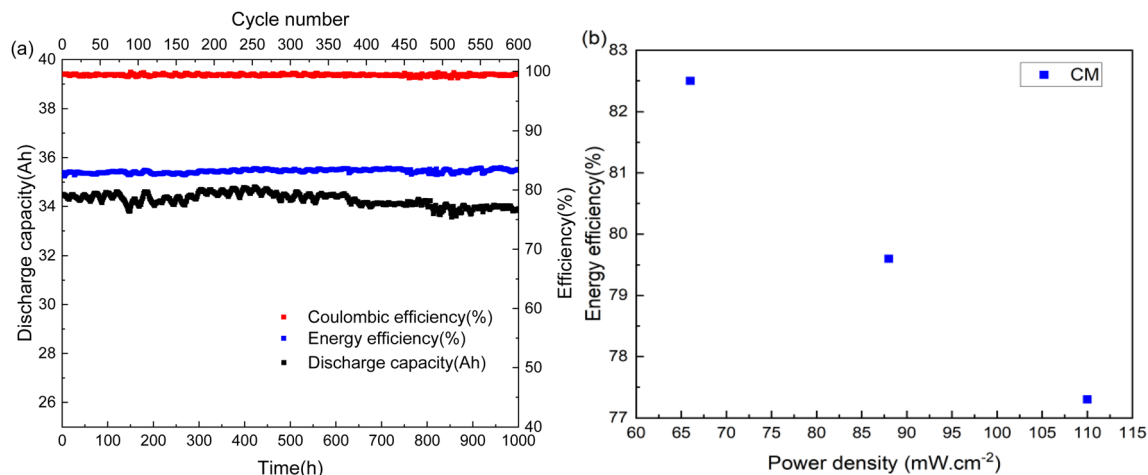
Fig. 4 (a) The electrochemical performance of the 52-stack cell assembled with the CM. (b) The EE for the 52-stack cell assembled with the CM at power densities of 66, 88 and 110 \text{mW cm}^{-2} .
