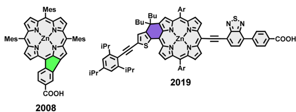
Fig. 2 Examples from literature on the application of five- and six-ring fused porphyrins in solar cells.
