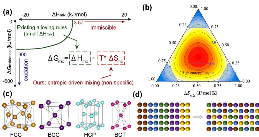
Fig. 1 (a) Enabling more alloy choices based on the entropic contribution ( -T\Delta S_{mix} ). Reproduced with permission. 32 Copyright 2021, Elsevier Ltd. (b) Different spaces of traditional alloy and high entropy alloy. Reproduced with permission. 33 Copyright 2016, Elsevier Ltd. (c) HEAs structure model. Reproduced with permission. 32 Copyright 2021, Elsevier Ltd. (d) High entropy effect.
