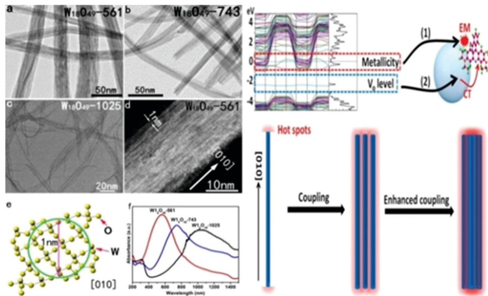
Fig. 21 (a–c) TEM images of W_{18}O_{49} -561, W_{18}O_{49} -743, and W_{18}O_{49} -1025, distinguished due to various in their LSPR peaks. (d) HRTEM image of W_{18}O_{49} . (e) Cross-section of a 1.0 nm nanowire inside of one W_{18}O_{49} unit cell oriented along the [010] direction. (f) UV-visible-NIR absorption spectra of the W_{18}O_{49} -561, W_{18}O_{49} -743, and W_{18}O_{49} -1025. (left) Top: Band structure of W_{18}O_{49} and the two possible SERS enhancement ways in W_{18}O_{49} : (1) EM and (2) CT. Bottom: LSPR coupling between nanowires. Adopted from ref.341 Copyright©2018, ACS.
