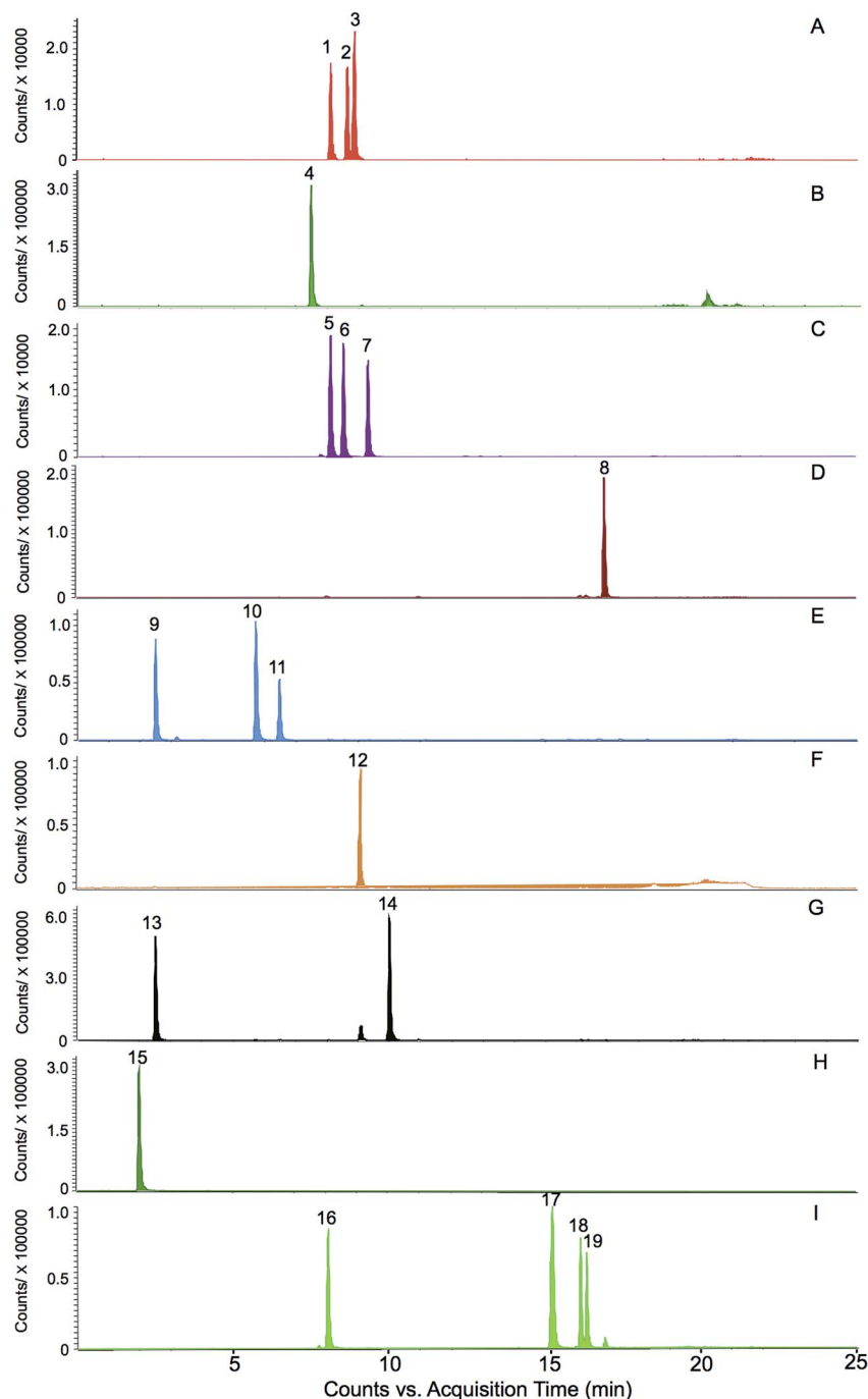
Fig. 2 The SIM scan spectrum of the 19 ginsenosides included six groups of isomers. (A) m/z 583.29 (1, R c ; 2, R b2 ; 3, R b3 ); (B) m/z 599.29 (4, R b1 ); (C) m/z 683.43 (5, 20(S)-Rh1; 6, 20(R)-Rh1; 7, F1); (D) m/z 793.43 (8, zingibroside R1); (E) m/z 845.49 (9, R g1 ; 10, F11; 11, R f ); (F) m/z 955.48 (12, R o ); (G) m/z 991.55 (13 R e ; 14, R d ); (H) m/z 977.53 (15, notoginsenoside R1); (I) m/z 829.49 (16, R g2 ; 17, F2; 18, 20(S)-R g3 ; 19, 20(R)-R g3 ).
