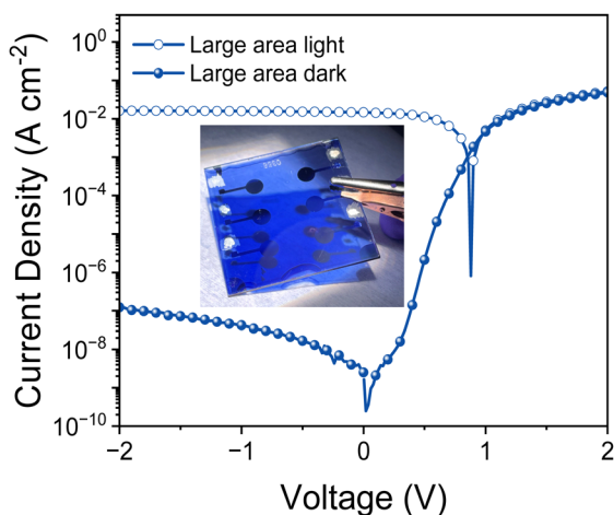
Fig. 5 (a) Current–voltage characteristics of large-area PTQ10:IDSe-based devices under AM1.5G illumination and dark; in inset the picture of the large-area device ( 5 \times 5 \text{ cm} substrates).
