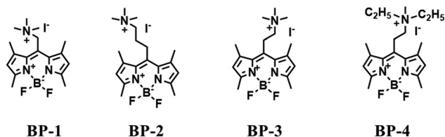
Fig. 24 The structures of dyes BP-1 , BP-2 , BP-3 , and BP-4 .
