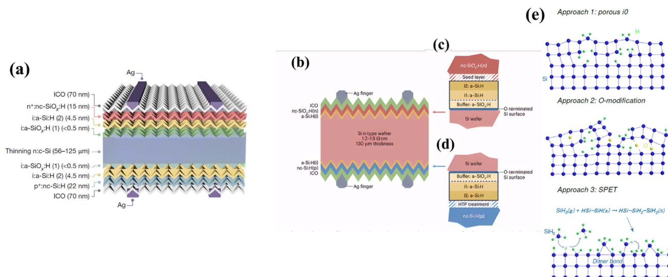
Fig. 9 (a) Structure schematics of the flexible SHJ solar cells with a two-stage composite gradient passivation process (reproduced from ref. 37 with permission from Springer Nature, copyright 2024). (b) Device structure of the solar cell with an efficiency of 26.81%. (c and d) Schematic representation of the front and rear surface fields (reproduced from ref. 83 with permission from Springer Nature, copyright 2023). (e) Three approaches for epitaxy growth suppression, which is a sandwiched passivation layer (i0/i1/i2), with an H-rich porous first layer (i0), deposited on oxygen-modified c-Si surface (reproduced from ref. 21 with permission from Springer Nature, copyright 2024).
