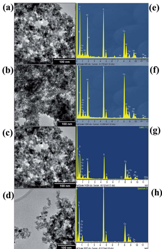
Fig. 3 TEM images of (a) TWZ703, (b) TWZ712, (c) TWZ721 and (d) TWZ730. EDS spectrum of (e) TWZ703, (f) TWZ712, (g) TWZ721 and (h) TWZ730.
