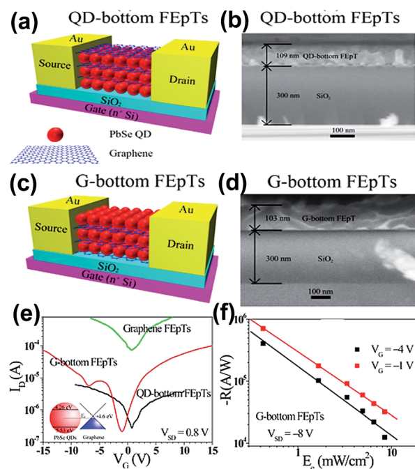
Fig. 9 Schematic diagram of QD at the bottom layer FETs (a) and the corresponding cross-sectional SEM images of the multi-heterojunction channel (b). Schematic diagram of graphene at the bottom layer of FETs (c) and the corresponding cross-sectional SEM images of the multi-heterojunction channel (d). (e) Transfer characteristics of Graphene FETs, G-bottom FETs and QD-bottom FETs without light illumination. (f) Responsivity as a function of illumination of the G-bottom FETs. Reprinted with permission from ref. 65. Copyright 2015 American Chemical Society.
