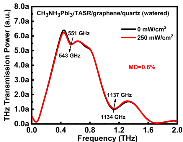
Fig. 8 Frequency-domain THz transmission by the \text{CH}_3\text{NH}_3\text{PbI}_3/\text{TASR}/\text{graphene}/\text{quartz} (watered) sample without photoexcitation (black) and excited by a 780 nm continuous-wave laser at 250 \text{ mW cm}^{-2} (red).
