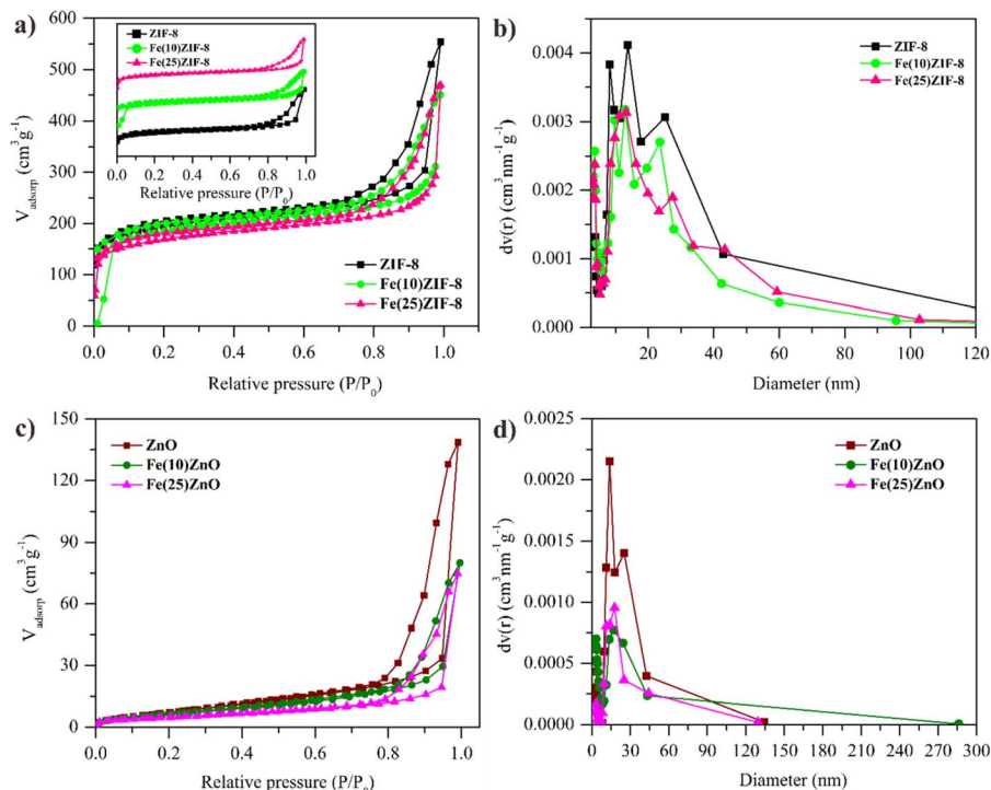
Fig. 5 N_2 adsorption–desorption isotherm of (a) MOF composites (c) MOF-derived metal oxide and BJH pore distribution of (b) MOF composites (d) MOF-derived metal oxide.
