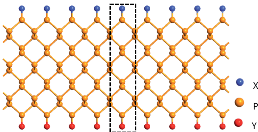
Fig. 1 The geometrical structures of the nonmetallic atom terminated ZPNRs, denoted as X-ZPNR-Y (X, Y = H, F, C, N, O, S, and Si). The black dotted rectangle exhibits a minimum repeated unit (supercell) used in this work.
