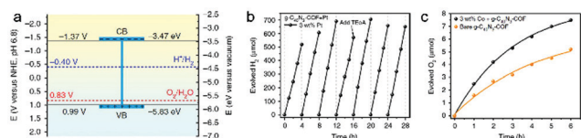
Fig. 24 (a) Bandgap diagram with marked potential for HER and OER. (b) Hydrogen and (c) oxygen production during photocatalytic water splitting based on g\text{-C}_{40}\text{N}_3\text{-COF} . Reproduced with permission. 27 Copyright 2019, Nature Publishing Group.
