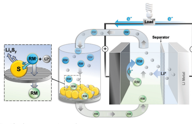
Fig. 12 Schematic of a Li-S RFB operating under discharge, highlighting the fundamental charge transfer steps between the RMs, electrodes and active material.
