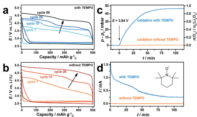
Fig. 7 Cycling profiles of \text{Li}-\text{O}_2 cells: (a) with, and; (b) without TEMPO, showing the decrease in charge potential when employing a redox mediator; (c) TEMPO redox shuttling was confirmed by oxidising \text{Li}_2\text{O}_2 sandwiched between separators ( i.e. disconnected from the electrode) by monitoring \text{O}_2 evolution, and; (d) the current, with and without TEMPO (orange and blue traces, respectively) while applying a potential of 3.84 V vs. \text{Li}^+/\text{Li} . Using the RM, \text{O}_2 evolution corresponding to formation of 92% of the maximum \text{Li}_2\text{O}_2 in the electrode was recorded. Adapted with permission from ref. 30. Copyright 2014 American Chemical Society.
