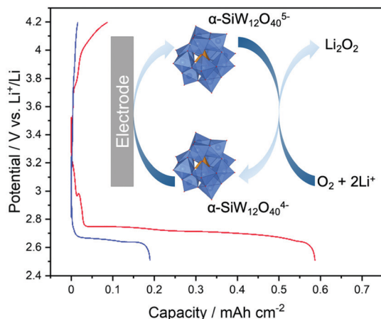
Fig. 4 Cycling profiles of a Li–O 2 cell containing [ \alpha -SiW 12 O 40 ] 4- (red trace) and a mediator-free cell (blue trace) showing a three-fold increase in discharge capacity when using the POM RM. Shown inset is the proposed mechanism of Li 2 O 2 formation using \alpha -SiW 12 O 40 4- as a mediator. Adapted from ref. 34 with permission from the Royal Society of Chemistry.
