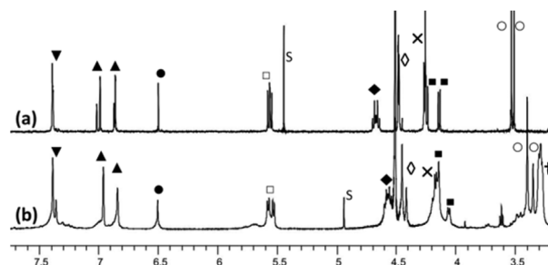
Fig. 1 ^1\text{H} NMR spectra (500 MHz, 300 K) of (a) organosoluble Rim 3 ligand in \text{CD}_3\text{CN} and (b) water-soluble WRim 3 ligand in \text{D}_2\text{O} (2.6 mmol). ( \blacktriangledown ) HAr. “down”; ( \blacktriangle ) HAr. “up”; ( \bullet ) \text{OCH}_2\text{O} ; ( \blacklozenge ) -\text{CHAr} ; ( \diamond ) \text{CH}_2\text{Im} ; ( \times ) \text{ArCH}_2\text{O} ; ( \circ ) \text{NCH}_3 ; ( \blacklozenge ) -\text{CHAr} ; ( \dagger ) \text{CH}_2\text{N}^+\text{Me}_3 . S stands for solvent.
