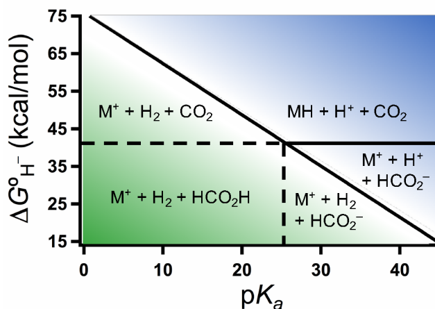
Figure 9. Regions of predicted metal hydride reactivity with \text{CO}_2 and \text{H}^+ as a function of \Delta G^\circ_{\text{H}^-} and \text{p}K_a . Adapted from reference 25.
