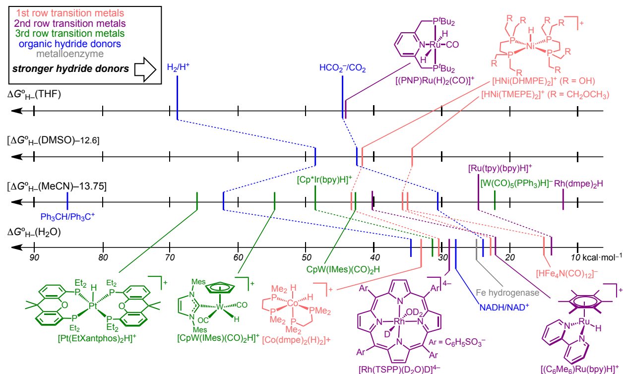
Figure 8. Comparing thermodynamic hydricity values of selected transition-metal-, organic-, and enzyme-based hydride donors in water (H 2 O), acetonitrile (MeCN), dimethyl sulfoxide (DMSO), and tetrahydrofuran (THF). As a result of differences in convention for the construction of scales, correction factors of 12.6 (DMSO) and 13.75 (MeCN) are applied to provide accurate comparisons of how hydricity changes across solvents. Within any given solvent, the relative values are not affected by the correction factors. See ESI for a complete table of hydricity values.
