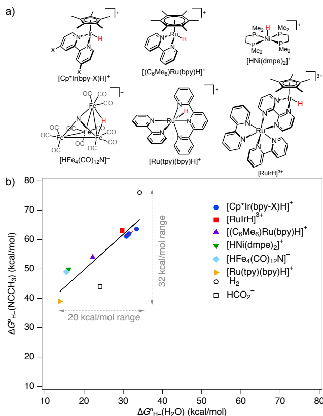
Figure 6. (a) Structures for a series of transition metal complexes with reported hydricities in both acetonitrile and water. (b) Aqueous hydricity values, \Delta G^\circ_{\text{H}-(\text{OH}_2)} , plotted versus corrected acetonitrile hydricity values, \Delta G^\circ_{\text{H}-(\text{NCCH}_3)} . Linear fits are provided for the full set of complexes (solid black line) as well as a family of iridium complexes (dashed red line). Adapted from reference 9.
