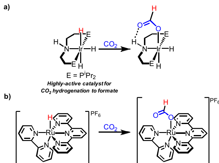
Figure 21. (a) Catalytically relevant CO_2 insertion into an unstable iridium complex and (b) model ruthenium complex used in stoichiometric studies for determining information related to kinetic hydricity.
