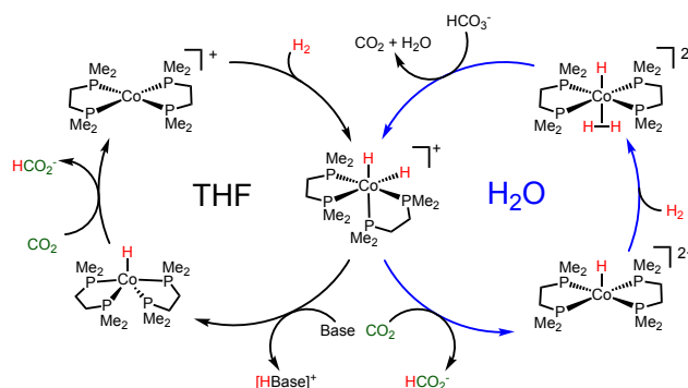
Figure 11. Catalytic reduction of \text{CO}_2 by [(\text{H})_2\text{Co}(\text{dmpe})_2]^+ in THF and \text{H}_2\text{O} . Hydride transfer occurs from \text{HCo}(\text{dmpe})_2 in THF, but from [(\text{H})_2\text{Co}(\text{dmpe})_2]^+ in water, due to solvent effects on hydricity.
