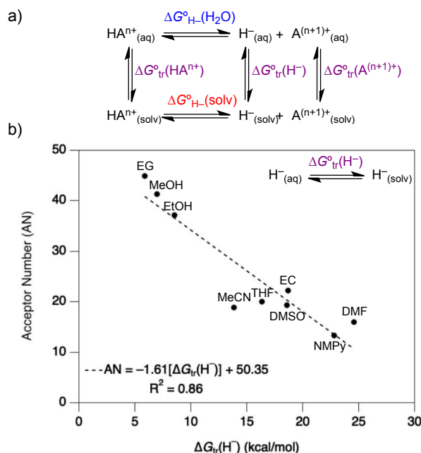
Figure 7. (a) General model for understanding how hydricity in water ( \Delta G^{\circ}_{\text{H}-(\text{H}_2\text{O})} ) differs from hydricity in organic solvent ( \Delta G^{\circ}_{\text{H}-(\text{solv})} ), based on the transfer free energy ( \Delta G^{\circ}_{\text{tr}} ) of each reactant and product. (b) Correlation between the transfer free energy of the hydride ion from water to organic solvents, \Delta G^{\circ}_{\text{tr}}(\text{H}^{-}) , and the acceptor number (AN) of the organic solvent. 9 Abbreviations: ethylene glycol (EG), methanol (MeOH), ethanol (EtOH), acetonitrile (MeCN), tetrahydrofuran (THF), ethylene carbonate (EC), dimethyl sulfoxide (DMSO), N-methyl-2-pyrrolidone (NMPy), dimethylformamide (DMF). Adapted from reference 9.
