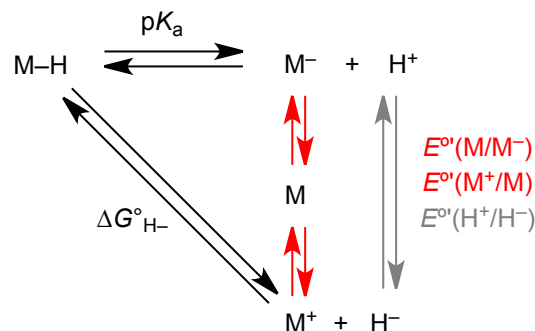
Figure 3. Thermochemical scheme for determining thermodynamic hydricity using the potential– pK_a method.
