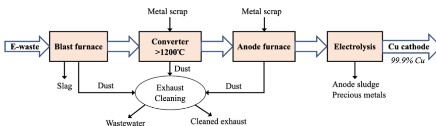
Fig. 12 Pyrometallurgical processing scheme based on industrial copper/e-waste smelting process. Adapted from ref. 55,86
