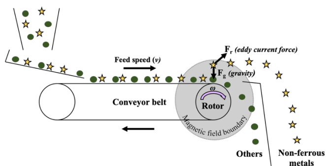
Fig. 7 Schematic of eddy current separation of non-ferrous metals from other components (metals, NMF).
