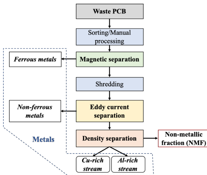
Fig. 6 Physical separation scheme for separation of NMF from metals.
