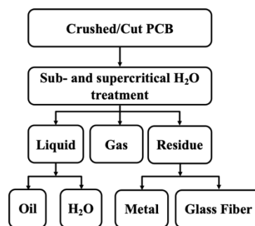
Fig. 9 Overview of sub- and supercritical water treatment methodology
