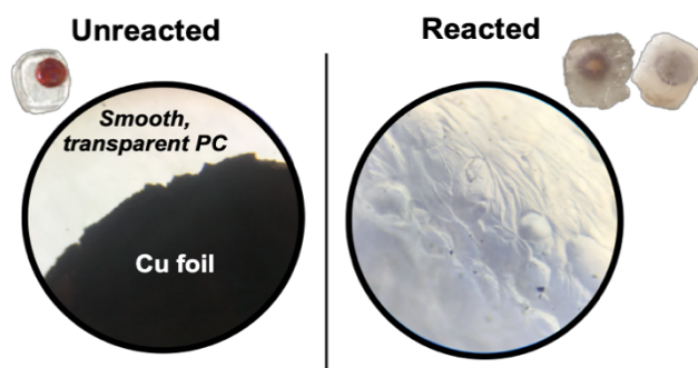
Fig. 18 A comparison of the unreacted control PCB particle (Cu in PC) and the reacted control PCB particle (reaction in scCO 2 solvent system).
