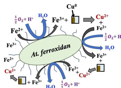
Fig. 16 The bioleaching mechanism of At. ferroxidans in solution with shredded PCB.
