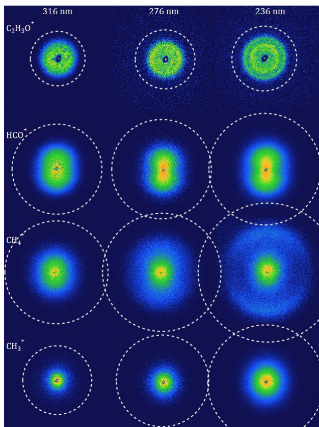
Figure 5 C_2H_3O^+ , HCO^+ , CH_4^+ , and CH_3^+ ion images (top to bottom) following photolysis of CH_3CHO^+ at 316 nm, 276 nm, and 236 nm (left to right). Dashed circles represent the maximum possible speeds for each ionic fragment assuming the neutral co-fragments given in reactions I-IV. The C_2H_3O^+ images on the top row have been magnified by a factor of two to more clearly show the structure.
