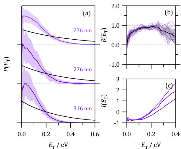
Figure 7 (a) HCO + total translational energy distributions at 316 nm, 276 nm, and 236 nm; (b) \beta(E_T) are shown for all photolysis wavelengths (316 – 228 nm) along with their average (black); (c) linear surprisal plots showing two distinct gradients.
