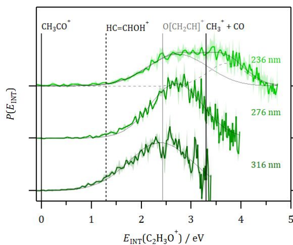
Figure 6 \text{C}_2\text{H}_3\text{O}^+ E_{\text{INT}} distributions at 316 nm, 276 nm, and 236 nm. Vertical lines are the energetic thresholds for formation of \text{CH}_3\text{CO}^+ isomers 1-hydroxyvinylum (dashed black) and vinylium (solid gray), along with secondary dissociation of \text{CH}_3\text{CO}^+ \rightarrow \text{CH}_3^+ + \text{CO} (solid black). Total fits are shown (solid black) along with individual components of the 236 nm E_{\text{INT}} distribution (solid and dashed black). The dashed component corresponds to formation of the 1-hydroxyvinylum isomer.
