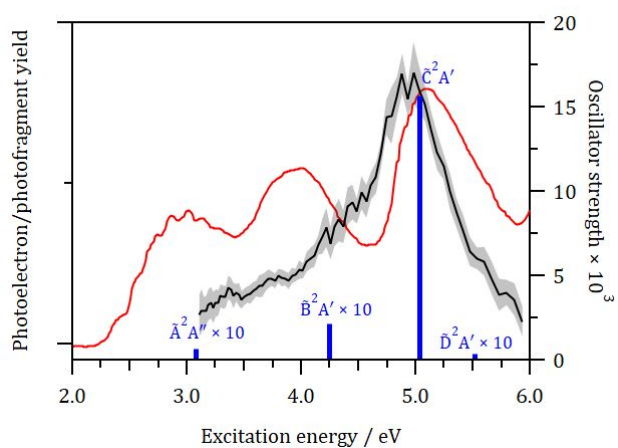
Figure 4 Total photofragment ion yield (black), photoelectron spectrum measured by Cvitaš et al. 28 (red), and oscillator strengths from EOM-CC(2,3)/cc-pVTZ calculations vs. vertical excitation energies (blue). Excitation energies are measured relative to the ground state of the \text{CH}_3\text{CHO}^+ cation; the photoelectron spectrum has been shifted by -10.23 eV.
