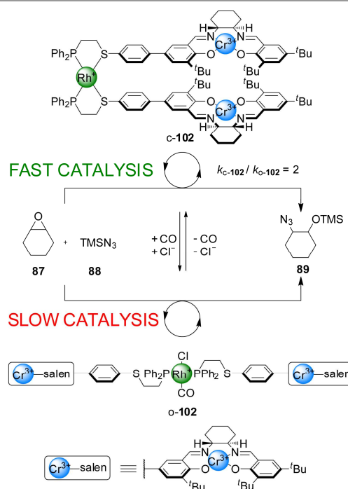
Scheme 27. Coordination-driven switching of the activity of tweezer catalyst o/c-102 . 51
