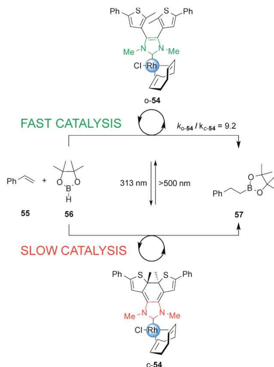
Scheme 8 Controlling the rate of a hydroboration reaction using switchable rhodium catalyst o/c-54. 29
