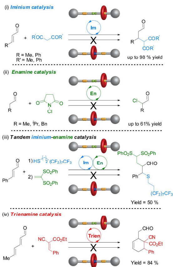
Figure 1. The scope of switchable rotaxane organocatalyst 72 through different activation mechanisms. 39
