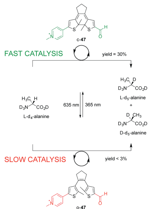
Scheme 6. Controlling the rate of the racemization of L-alanine using switchable catalyst o/c-47 . 26
