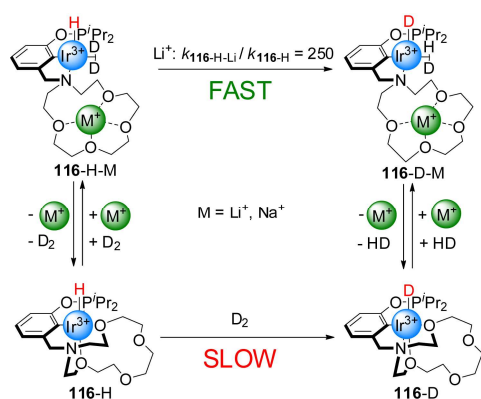
Scheme 31. \text{D}_2 activation by Ir(III) catalyst 116 triggered by reversible coordination of an alkali metal cation to a crown ether ligand. 62
