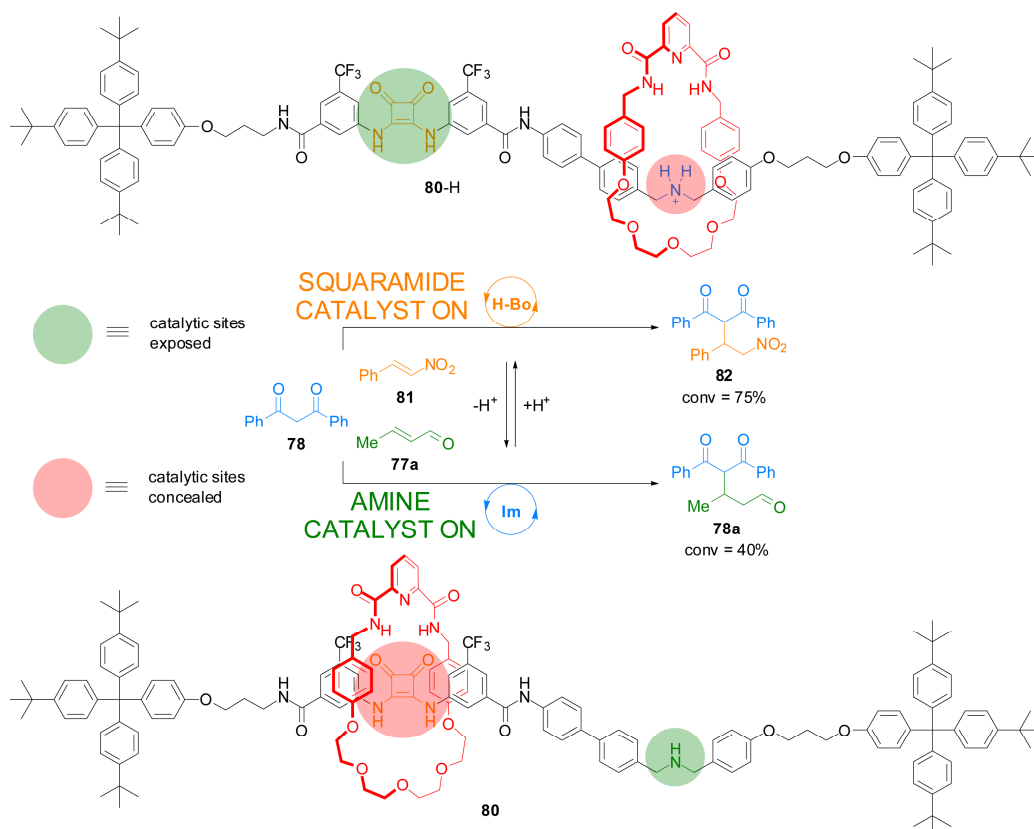
Scheme 11. Controlling the reaction outcome from a mixture of building blocks using a switchable rotaxane featuring two different organocatalytic sites, 80 . 41
