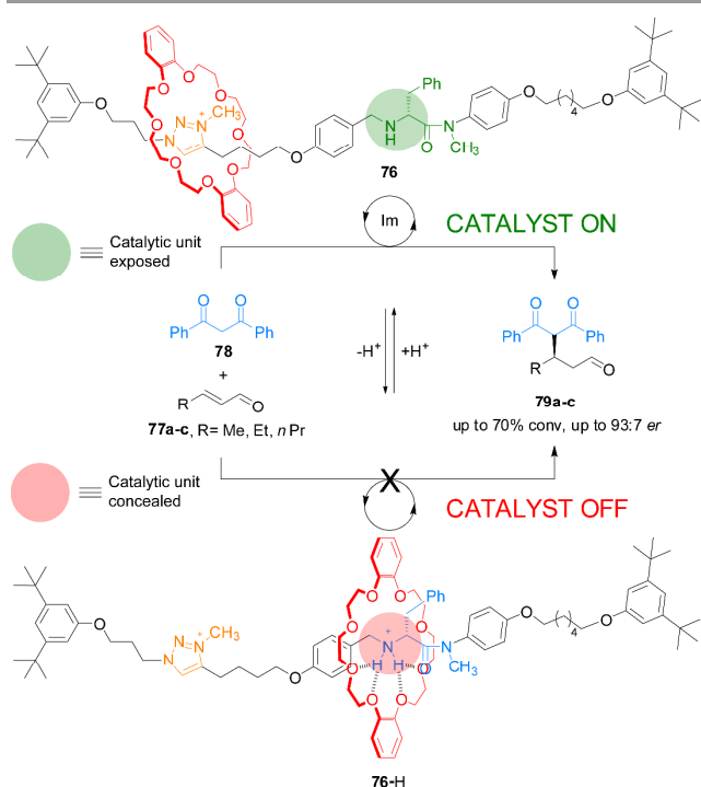
Scheme 10. Controlling the rate and stereoselectivity of Michael addition using a switchable rotaxane asymmetric organocatalyst 76 . 40
