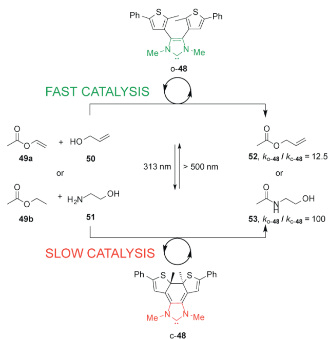
Scheme 7. Controlling the rate of transesterification and amidation reactions using switchable catalyst o/c-48. 27
