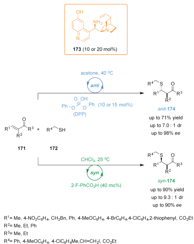
Scheme 52. Solvent- and acid-dependent diastereodivergent Michael addition of alkyl thiols to \alpha,\beta -unsaturated ketones catalyzed by cinchona alkaloid derivative 173 . 98
