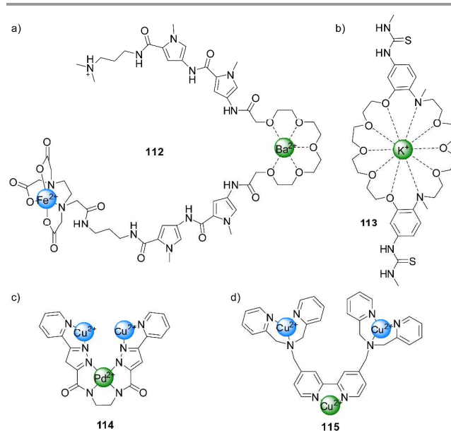
Figure 2. Catalysts activated by conformational changes induced by coordination of metal ions. 56-61
