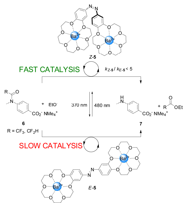
Scheme 2. Controlling the rate of anilide ethanolsis using photoswitchable catalyst E/Z -5. 9
