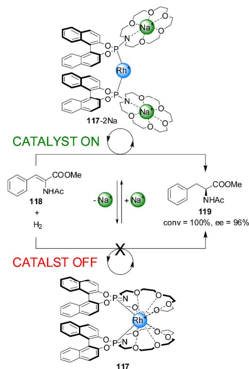
Scheme 32. 'On'-'off' switching of Rh(I) catalyst 117 driven by addition or removal of \text{Na}^+ ions. 63
