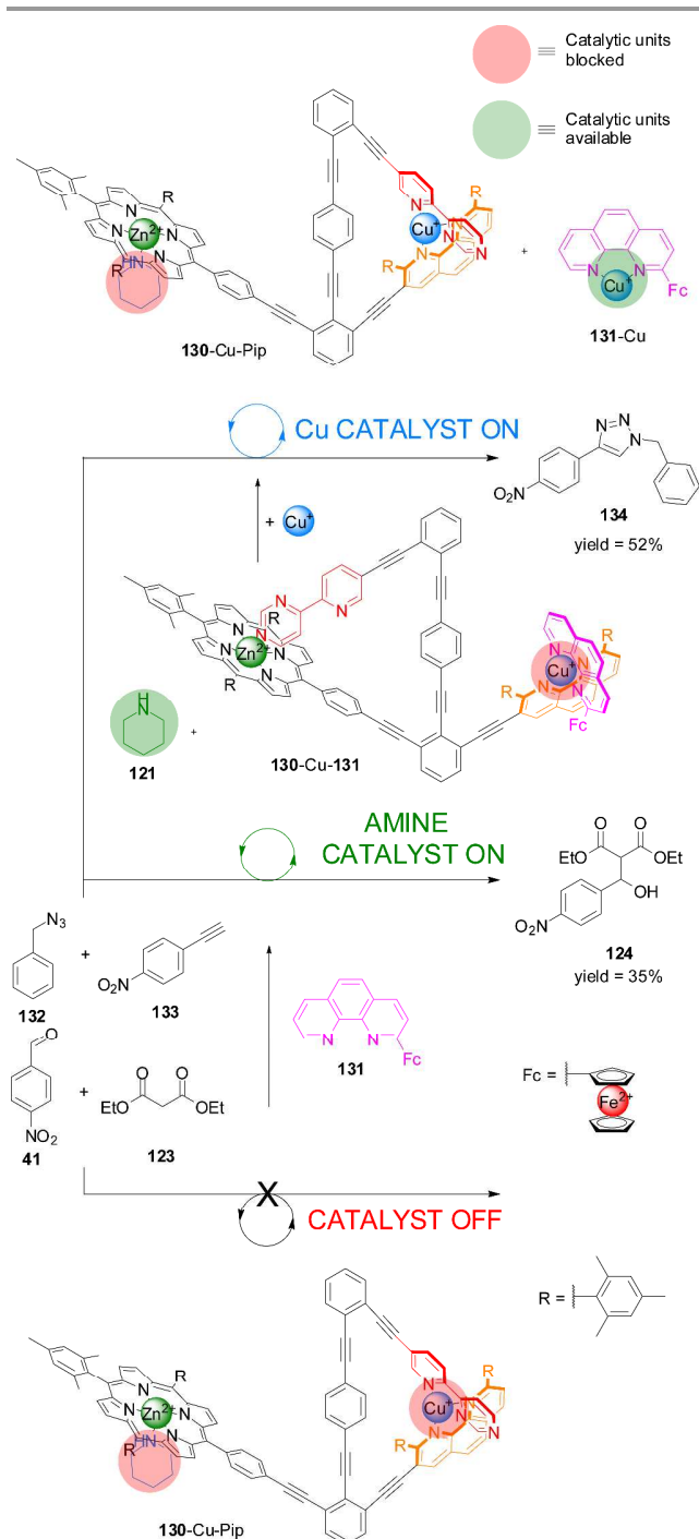
Scheme 36. Switching of catalytic system 130 between an 'off' state and two 'on' states with orthogonal catalytic processes through the sequential addition of phenanthroline derivative 131 and Cu(I). 67
