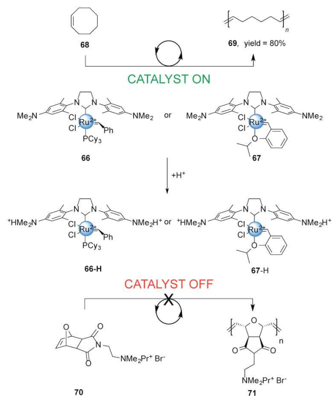
Scheme 9. Controlling the rate of ROMP using pH-switchable catalysts 66 and 67 . 33
