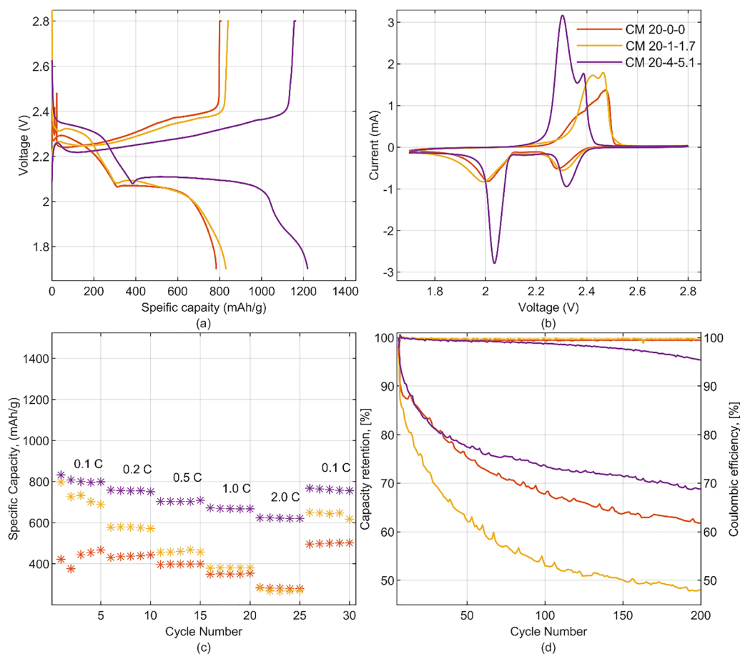
Fig. 7 Electrochemical test of the samples CM 20-0-0, CM 20-1-1.7 and CM 20-4-5.1, investigating materials prepared with different amounts of urea. (a) Formation at 0.1C, (b) cyclic voltammety at 0.05\text{ mV s}^{-1} , (c) current rate (0.2C charge current) and (d) cycle life tests at 0.2C. Electrolyte: 1 M LiTFSI with 2 wt% ( \text{LiNO}_3 ) in 1 : 1 DOL/DME, 15\text{ }\mu\text{L/1 mg} of sulfur.
