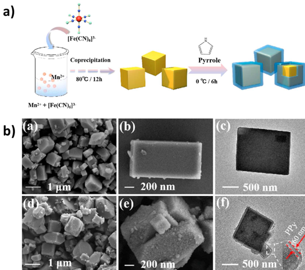
Fig. 16 (a) Schematic illustration of KMnCF and KMnCF@PPy sample. (b(a and b)) SEM and (c) TEM images of KMnCF. (d and e) SEM and (f) TEM images of KMnCF-30. Reprinted from ref. 54, copyright (2022), with permission from ACS.
