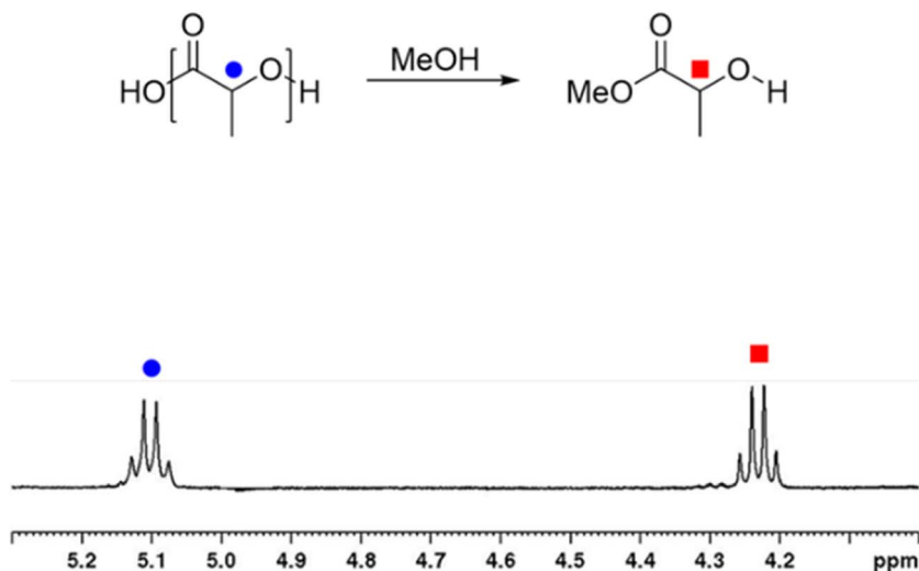
Fig. 1 ^1\text{H} NMR spectrum (600 MHz, \text{CDCl}_3 , 298 K) with methine group assignments for a PLLA methanolysis (NMR monitoring of entry 2 of Table 1 at 58% of conversion).
