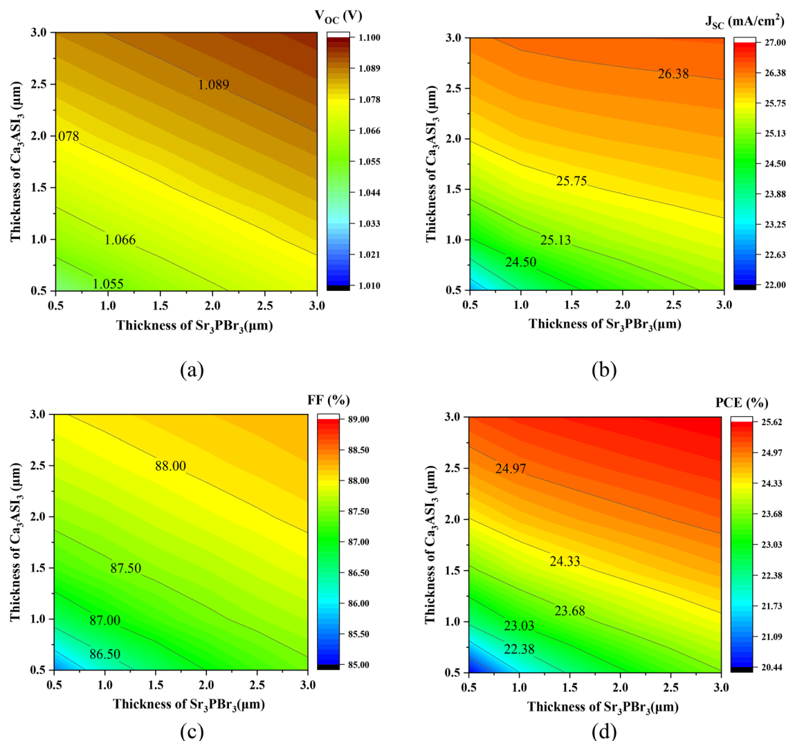
Fig. 3 Role of thickness variation of \text{Sr}_3\text{PBr}_3 and \text{Ca}_3\text{AsI}_3 (device-iii) on the photovoltaic parameters, (a) V_{\text{OC}} , (b) J_{\text{SC}} , (c) FF, and (d) PCE.
