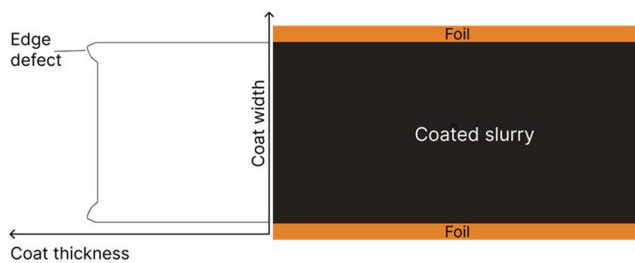
Fig. 7 Illustration of edge defect in an electrode slurry for continuous coating, superelevation at the edges of the coated slurry can be observed.
