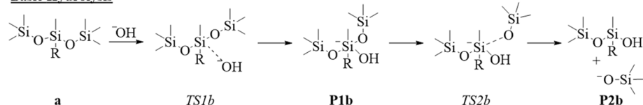
Scheme 1 Hydrolysis reactions for TriSil-1n (a) under neutral, acidic, and basic conditions. R represents the PEG chain. Energies for these reactions are presented in the potential energy diagram in Fig. 2.
