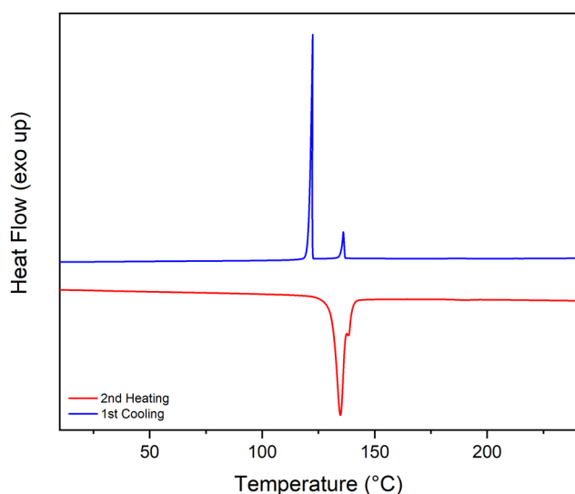
Fig. 3 DSC scan of 7b. Second heating curve (10 K min -1 ) is shown in red, first cooling curve (10 K min -1 ) in blue. Pseudo-monotropic behavior can be seen in the red heating curve.
