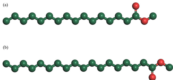
Fig. 8 Schematic diagram of the structures of (a) methyl palmitate (MP) and (b) methyl stearate (MS).
