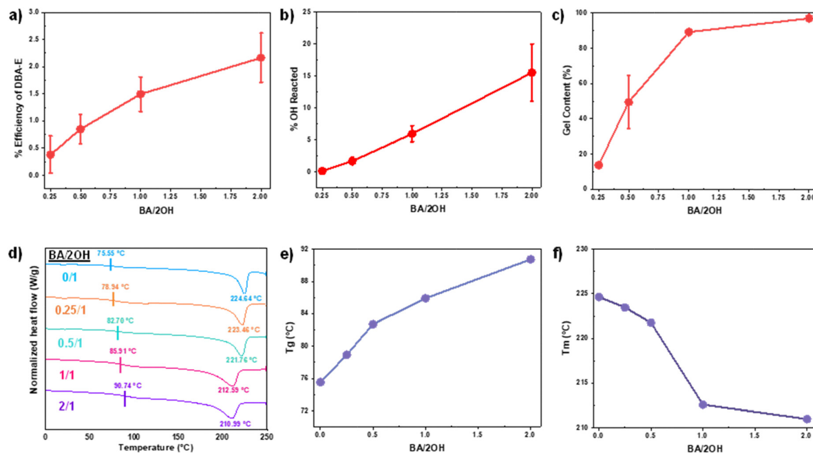
Fig. 4 Effect of the amount of DBA-E as the mole equivalent ratio of BA/2OH using gravimetry on the % efficiency of DBA-E incorporated into fibers (a), %OH reacted with DBA-E (b), and gel content as %insoluble species of BE-PVA mats in water (c); overlaid DSC thermograms (d) and thermal properties as T_g (e) and T_m (f) for BE-PVA mats fabricated with various amount of DBA-E as the mole equivalent ratio of BA/2OH.
