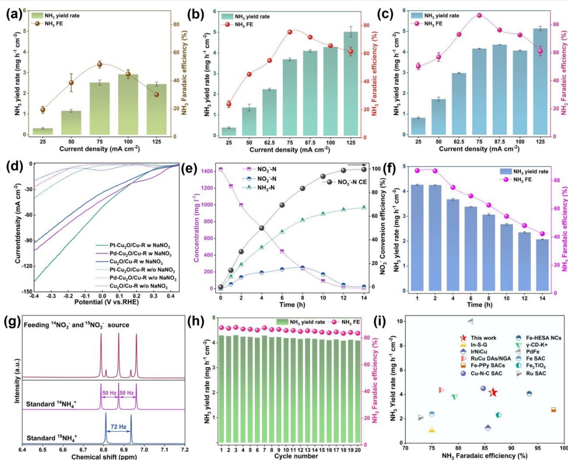
Fig. 4. Potentiostatic \text{NO}_3\text{RR} : The \text{NH}_3\text{-N} yield rate, FE of (a) \text{Cu}_2\text{O}/\text{Cu-R} ; (b) \text{Pd-Cu}_2\text{O}/\text{Cu-R} and (c) \text{Pt-Cu}_2\text{O}/\text{Cu-R} ; (d) LSV curves of \text{Cu}_2\text{O}/\text{Cu-R} , \text{Pd-Cu}_2\text{O}/\text{Cu-R} and \text{Pt-Cu}_2\text{O}/\text{Cu-R} without, and with, \text{NO}_3^- in 0.1M NaOH; Time-dependent variation of (e) \text{NO}_3^- , \text{NO}_2^- , \text{NH}_3\text{-N} concentration, \text{NO}_3\text{-N} CE; and (f) \text{NH}_3\text{-N} yield rate, FE during \text{NO}_3\text{RR} ; (g) ^1\text{H} NMR spectra of \text{Pt-Cu}_2\text{O}/\text{Cu-R} after \text{NO}_3\text{RR} using ^{14}\text{NO}_3^- and ^{15}\text{NO}_3^- ; (h) Stability test of \text{NO}_3\text{RR} for \text{Pt-Cu}_2\text{O}/\text{Cu-R} ; (i) Specific \text{NH}_3\text{-N} yield rate of previously reported systems with different FE for the \text{NO}_3\text{RR} .
