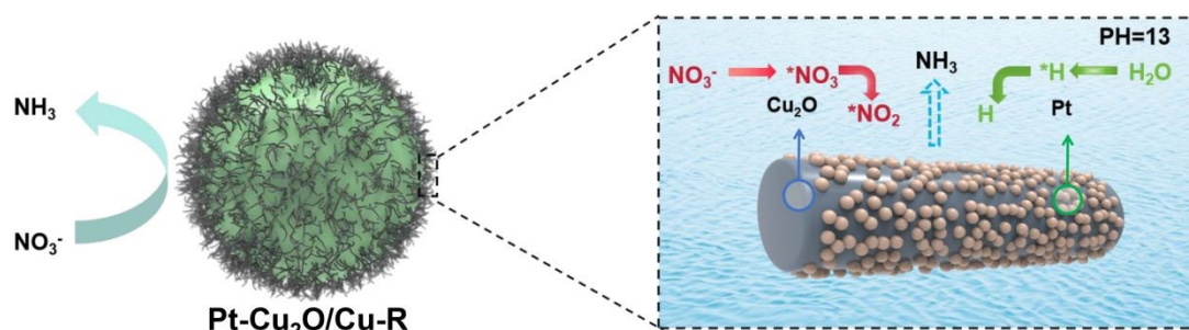
Fig. 7. Schematic representation of the \text{NO}_3\text{RR} of active sites on the surface of \text{Pt-Cu}_2\text{O/Cu-R} electrode at pH 13. This schematic integrates the key experimental findings of this work: the stabilization of \text{Cu}^+ sites, the critical role of atomic ^*\text{H} supplied from Pt-facilitated water dissociation, and the detection of key nitrogenous intermediates.
