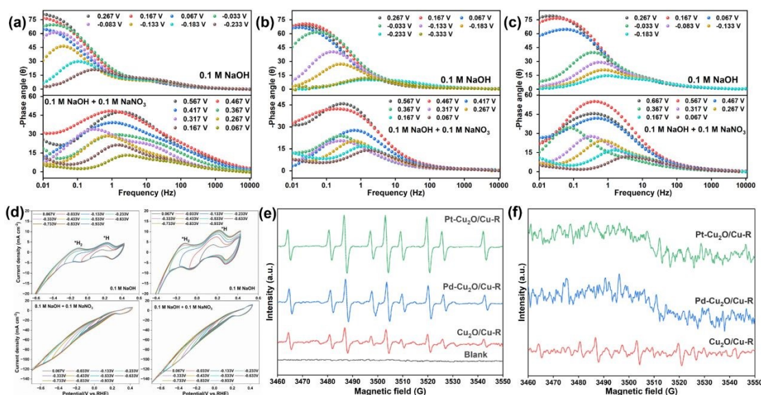
Fig. 5. Bode phase plots of (a) Cu 2 O/Cu-R; (b) Pd-Cu 2 O/Cu-R and (c) Pt-Cu 2 O/Cu-R in different electrolytes at various electrochemical; (d) CV curves of (left) Cu 2 O/Cu-R and (right) Pd-Cu 2 O/Cu-R in 0.1 M NaOH, with or without addition of 0.1 M NO 3 - ; (e) EPR spectra of the Cu 2 O/Cu-R, Pd-Cu 2 O/Cu-R and Pt-Cu 2 O/Cu-R in 0.1 M NaOH; (f) EPR spectra with added NO 3 - .
