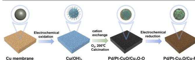
Fig. 1. Schematic illustration of the fabrication process of Pd/Pt-Cu 2 O/Cu-R membrane.
