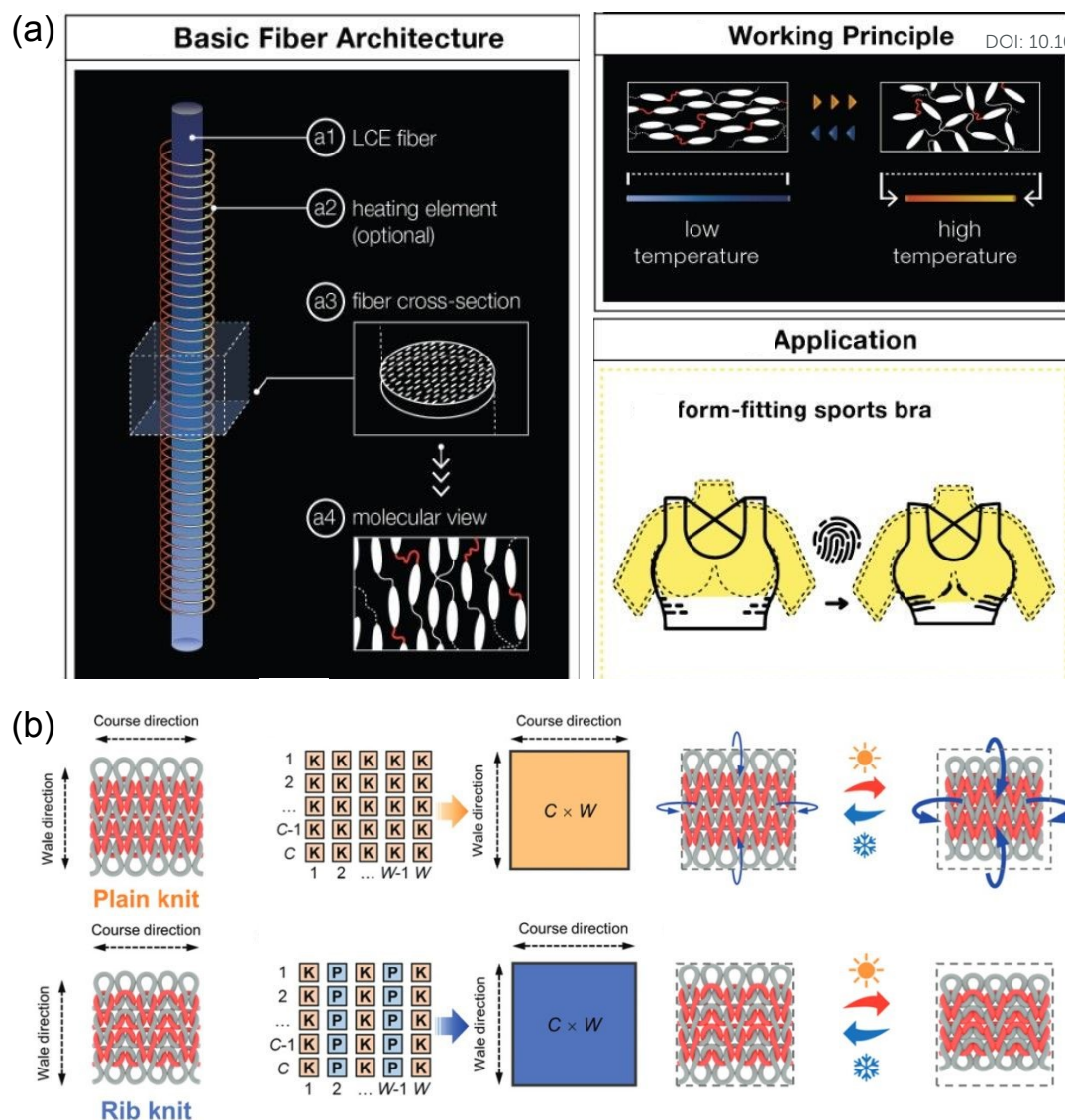
Fig. 9. LCE-based textile actuators. (a) Architecture and working principle of FibeRobo fibers and application in form-fitting sports bras. Reproduced with permission. 208 Copyright 2023, Association for Computing Machinery. (b) Thermal deformation of LCE actuators with knit and rib-knit patterns. Reproduced with permission. 237 Copyright 2023, John Wiley and Sons.
