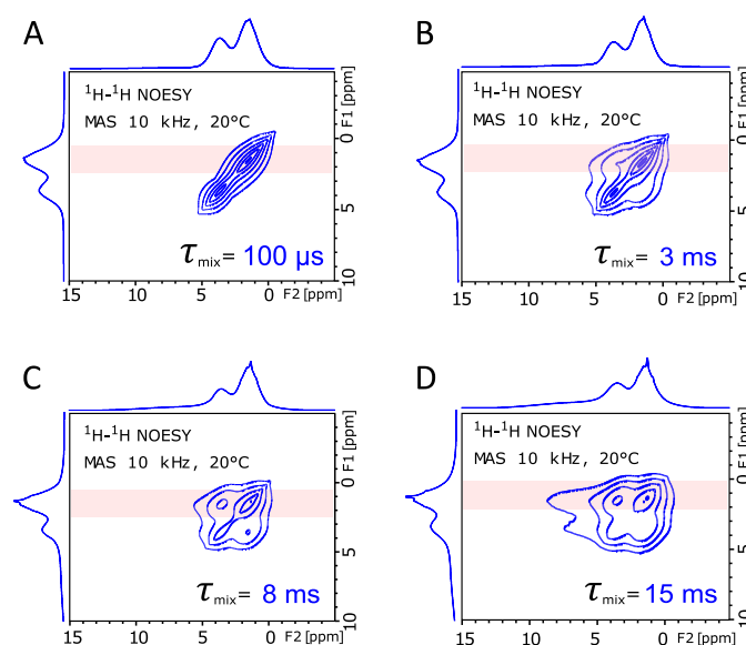
Figure 5: 2D ^1\text{H} – ^1\text{H} spin-diffusion spectra at different mixing times (MAS rate 10 kHz). The red-shaded region indicates the integration range along the indirect dimension (along y ) for the 1D projections shown in Figure 6A.
