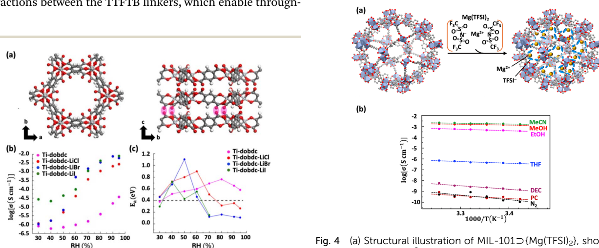
Fig. 3 (a) Structural model of the 2D-layered MOF Ti-dobdc, illustrating the hexagonal pore channels and highlighting in pink the non-coordinated carboxyl oxygen. (b) Ionic conductivity of Ti-dobdc and Ti-dobdc–LiX (X = Cl, Br, I) measured at 298 K under varying relative humidity (RH). (c) Corresponding activation energy values vs. RH. Adapted from ref. 46 with permission from Wiley-VCH, copyright 2023.
