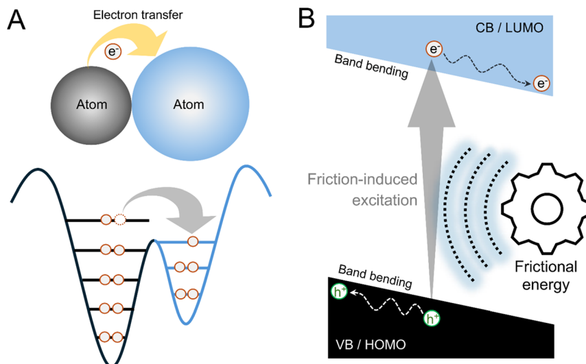
Fig. 1 Schematic of the mechanisms of tribocatalysis: (A) electron transfer and (B) electron transition. Band bending is expected in a semi-conducting catalyst (B), especially near its surface, when exposed to frictional forces.
