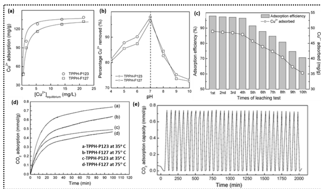
Fig. 14 (a) Cu 2+ adsorption isotherm for TPPH hybrid materials. (b) Effect of pH on Cu 2+ removal by the TPPH material. (c) Reusability of the adsorbent TPPH-P123 for Cu 2+ ions (10 mg L -1 ). (d) TGA records for CO 2 adsorption. (e) Multiple cycles of CO 2 adsorption measurements. Adapted with permission from ref. 61 Copyright of Royal Society of Chemistry, 2010.
