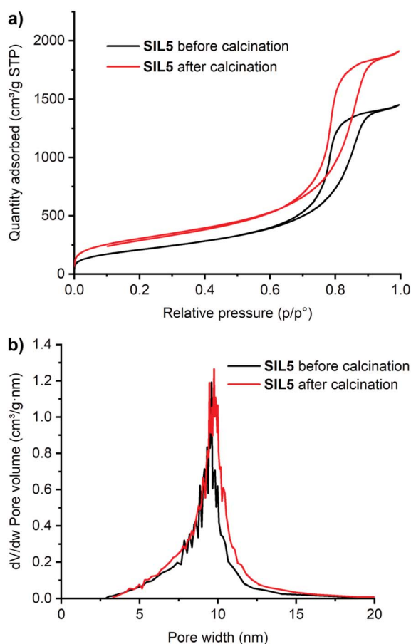
Fig. 1 (a) \text{N}_2 adsorption/desorption isotherms of SIL5 before (black line) and after calcination (red line) and (b) pore size distribution as \text{dV}/\text{dw} ( \text{cm}^3 \text{ g}^{-1} \cdot \text{nm}^{-1} ) vs. pore width (nm) calculated by the Barrett–Joyner–Halenda (BJH) model of SIL5 before (black line) and after calcination (red line).
