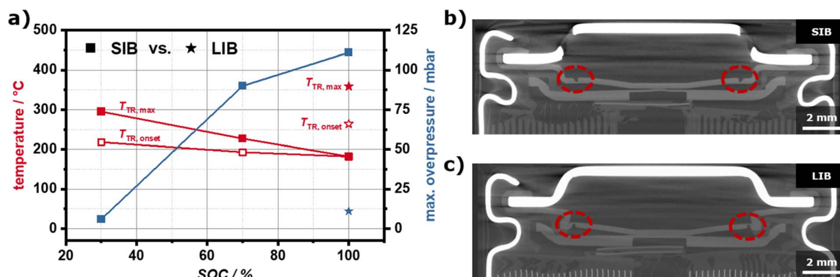
Fig. 3 (a) Summary of the SOC-dependent TR-behaviour, by means of T_{TR, onset} , T_{TR, max} and p_{max} of the SIB- and LIB-cells investigated. The T_{TR, max} -values of the SIB-cells at 70% SOC and 100% SOC are not reasonable due to the strong jelly roll ejection at these SOC. CT-images of the top of (b) the SIB-cell and (c) the LIB-cell.
