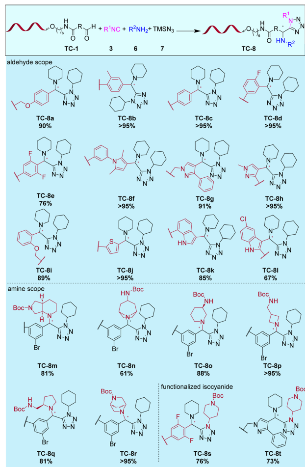
Fig. 4 Scope of the Ugi-azide four-component reaction on 10mer TC-DNA. Reaction conditions: TC-1 (3 nmol) and copolymer (90 nmol) and secondary amine 6 (6 μmol) in MeOH/CHCl 3 (50 μL; 3:1, v/v) for 3 h at rt. Addition of isocyanide 3 (6 μmol) and TMSN 3 7 (6 μmol). The reaction was run for 16 h at 50 °C.
