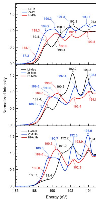
Fig. 7 B K-edge XAS spectra of [\text{M}(\text{RBH}_3)_4] complexes with \text{M} = \text{Zr} (blue) and \text{Hf} (red) and comparison to their corresponding \text{Li}(\text{RBH}_3) salts (black). Labeled positions indicate peak maxima in the spectra or peak positions identified by analysis of the second derivative traces (Fig. S51–S53; SI).
