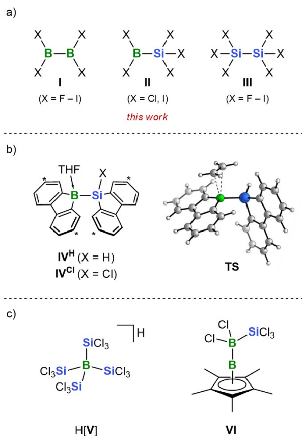
Fig. 1 (a) Perhalogenated diboranes(4) ( I ), disilanes ( III ), and the perhalogenated silylboranes ( II ) studied in this work. (b) Previously studied silylboranes ( IV ) capable of undergoing uncatalyzed silaboration reactions (C atoms marked with asterisks bear t Bu substituents); computed transition state ( TS ) for the silaboration of ethylene with IV H ( t Bu groups have been omitted in the calculations). (c) Silylborates H[V] and VI bearing some structural similarity with II .
