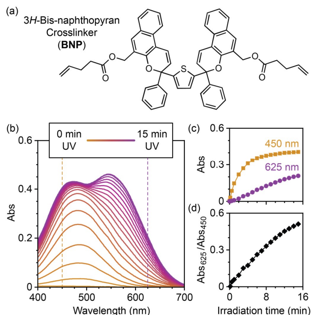
Figure 2. (a) Structure of the 3H-bis-naphthopyran crosslinker (BNP) used in this study. (b) UV-vis absorption spectra acquired during the photoirradiation (311 nm, 15 min) of a solution of BNP in THF (8 µg/mL, 30 mM BHT, -78 °C). (c) Absorbance at 450 nm and 625 nm as a function of photoirradiation time. (d) Ratio of the absorbance at 625 nm and 450 nm as a function of photoirradiation time.
