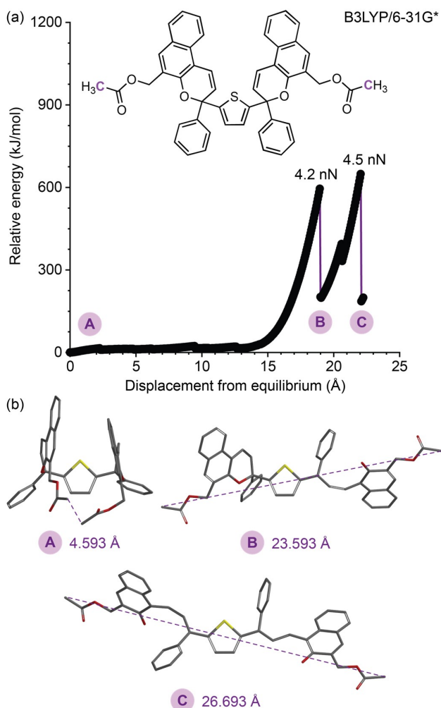
Figure 1. (a) Density functional theory (DFT) calculations using the constrained geometries simulate external force (CoGEF) method performed on a truncated model of the 3H-bis-naphthopyran mechanophore predict the expected ring-opening reactions to generate mono-merocyanine and bis-merocyanine products. Calculations were performed at the B3LYP/6-31G* level of theory. (b) The corresponding computed structures of the truncated molecule at various points of elongation are shown along with the associated constraint distance between the terminal carbon atoms. Data for the (R,S) diastereomer shown (see the ESI for additional information).
