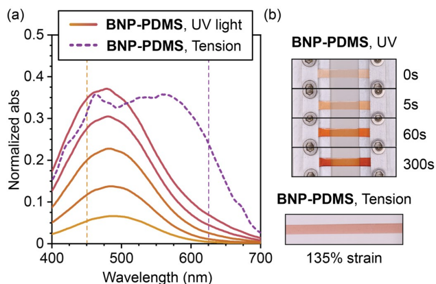
Figure 4. (a) Absorption spectra of BNP-PDMS after 5 s, 30 s, 60 s, 120 s, and 300 s of photoirradiation with 311 nm UV light compared to a sample of BNP-PDMS at 135% strain. (b) Photographs of BNP-PDMS after 0 s, 5 s, 60 s, and 300 s of photoirradiation with UV light compared to a sample of BNP-PDMS at 135% strain.
