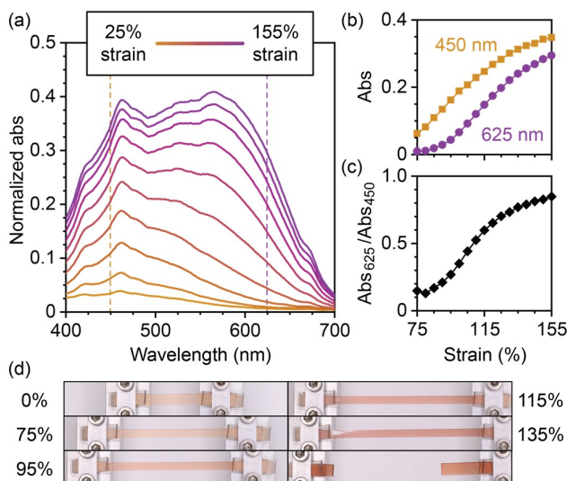
Figure 3. (a) Normalized UV-vis absorption spectra acquired during uniaxial tensile loading of BNP-PDMS . (b) Absorbance at 450 nm and 625 nm as a function of strain. (c) Ratio of the absorbance at 625 nm versus 450 nm as a function of strain. (d) Photographs of a different sample of BNP-PDMS at various strain values. The sample failed between 135 and 140% strain.
