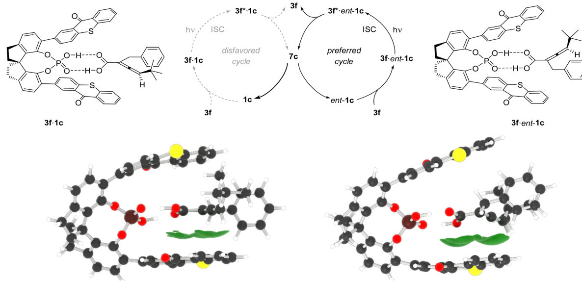
Scheme 7 Mechanistic scenario for the deracemization of racemic allenic acid rac -1c upon irradiation in the presence of catalyst 3f . Triplet energy transfer is faster in complex 3f-ent-1c than in complex 3f-1c because the average distance of the thioxanthone chromophore to the allene is smaller. Triplet energy transfer from excited 3f* to the allene leads to formation of achiral triplet intermediate 5c (cf. Scheme 6) which dissociates from the phosphoric acid and forms either one of the two enantiomers 1c or ent - 1c of the allenic acid. The lowest minimum energy conformations of each enantiomer with catalyst 3f are shown below, in addition to the overlap of scaled van der Waals radii (green areas) to visualize the proximity of the allenic acids to the catalyst.
