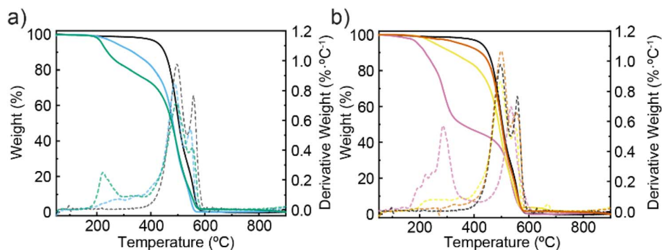
Fig. 2 (a) TGA analysis (air, 10 °C min -1 ) of (6,5)-SWNT (black), eW ⊃SWNT (green), and the mixture of 1 and 2 with (6,5)-SWNTs in the absence of cat. TFA (blue). (b) TGA analysis (air, 10 °C min -1 ) of (6,5)-SWNT (black), the supramolecular complexes formed by the combination of (6,5)-SWNTs and 1 (yellow) or 2 (orange) and the equimolar mixture of 1 and 2 in absence of (6,5)-SWNTs (pink).
