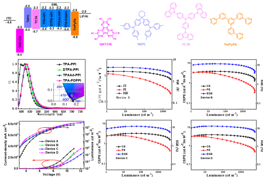
Fig. 5 Energy-level diagram and structure of the devices, chemical structure of the materials used in the OLEDs, voltage-dependent EL spectra of the devices based on TPA-PPI, DTPA-PPI, TPAAAd-PPI and TPA-POPPI, current density–voltage–luminance ( J – V – L ) characteristics and relationship between EL efficiencies and luminance for the devices.
