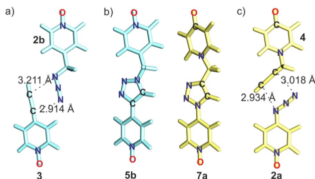
Fig. 3 (a) Arrangement of the reacting substrates in the energy-minimized structures of: (a) the ( 2b · 3 ) \subset 1 ternary hetero-complex and (c) the ( 2a · 4 ) \subset 1 ternary hetero-complex. The N_{\text{azide}}\text{--}C_{\text{acetylide}} distances are shown. (b) Energy-minimized structures of the 1,4-triazole isomers 5b (light-blue) and 7a (light-yellow) in the complexes 5b \subset 1 and 7a \subset 1 . For clarity the structure of cage 1 is not shown in the figures.
