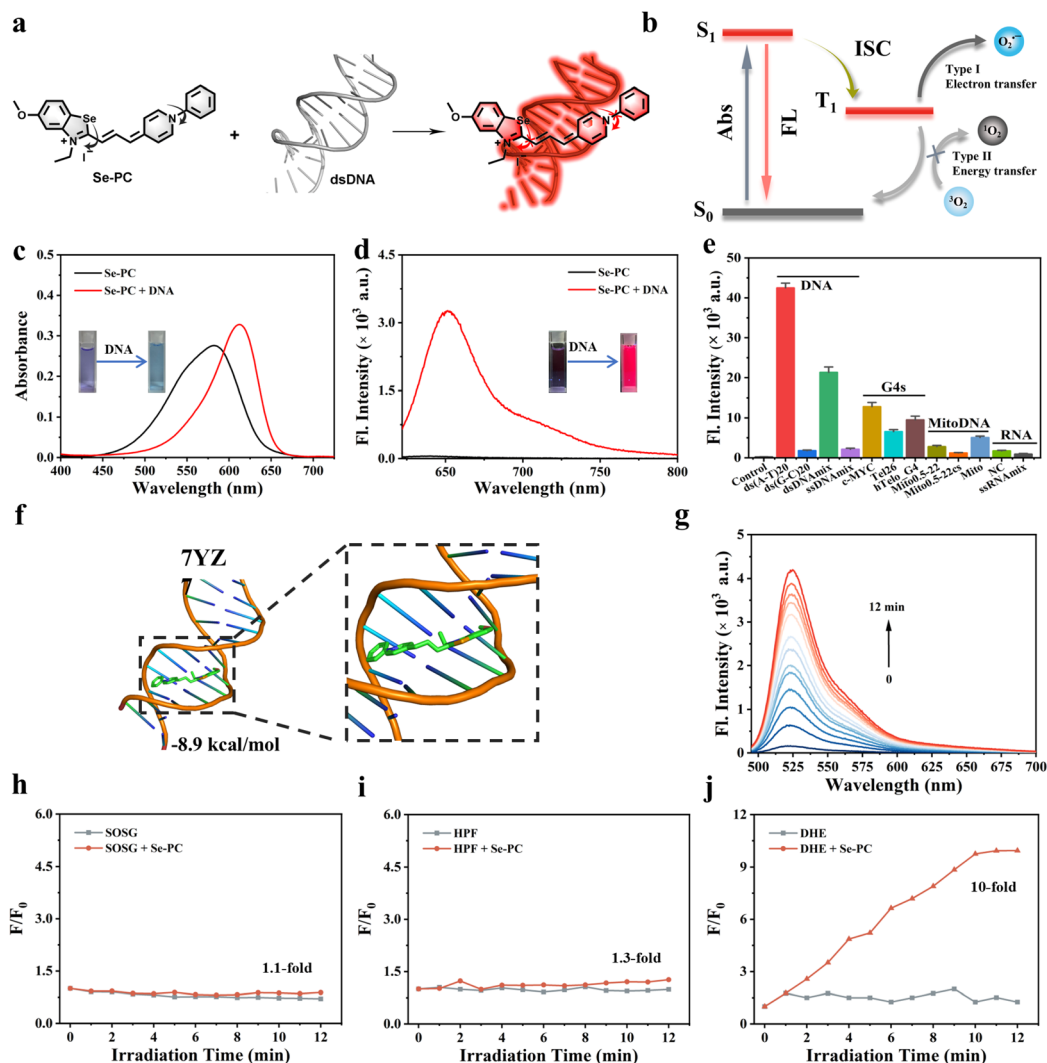
Fig. 1 (a) Schematic illustration of Se-PC binding to dsDNA. (b) The proposed mechanism for efficient photodynamic therapy. (c) UV-vis absorption spectra and (d) fluorescence spectra of Se-PC (4 \mu M) in the absence or presence of CT DNA (100 \mu g mL ^{-1} ) in 10 mM PBS buffer (300 mM NaCl, pH 7.4). (e) Fluorescence intensity of Se-PC (1.0 \mu M) at 650 nm in response to various oligonucleotides (4.0 \mu M). (f) Molecular docking calculation of Se-PC with dsDNA (7YZ, 111D, and 2GYX). (g) Fluorescence spectra of DCFH (10 \mu M) for Se-PC after irradiation (0.1 mW cm ^{-2} ) for different time periods. (h) Fluorescence intensities of SOSG (0.5 \mu M) at 525 nm, (i) fluorescence intensities of HPF (10 \mu g mL ^{-1} ) at 515 nm and (j) fluorescence intensities of DHE (10 \mu M) at 610 nm with irradiation (0.1 mW cm ^{-2} ) or without irradiation for different time periods.
