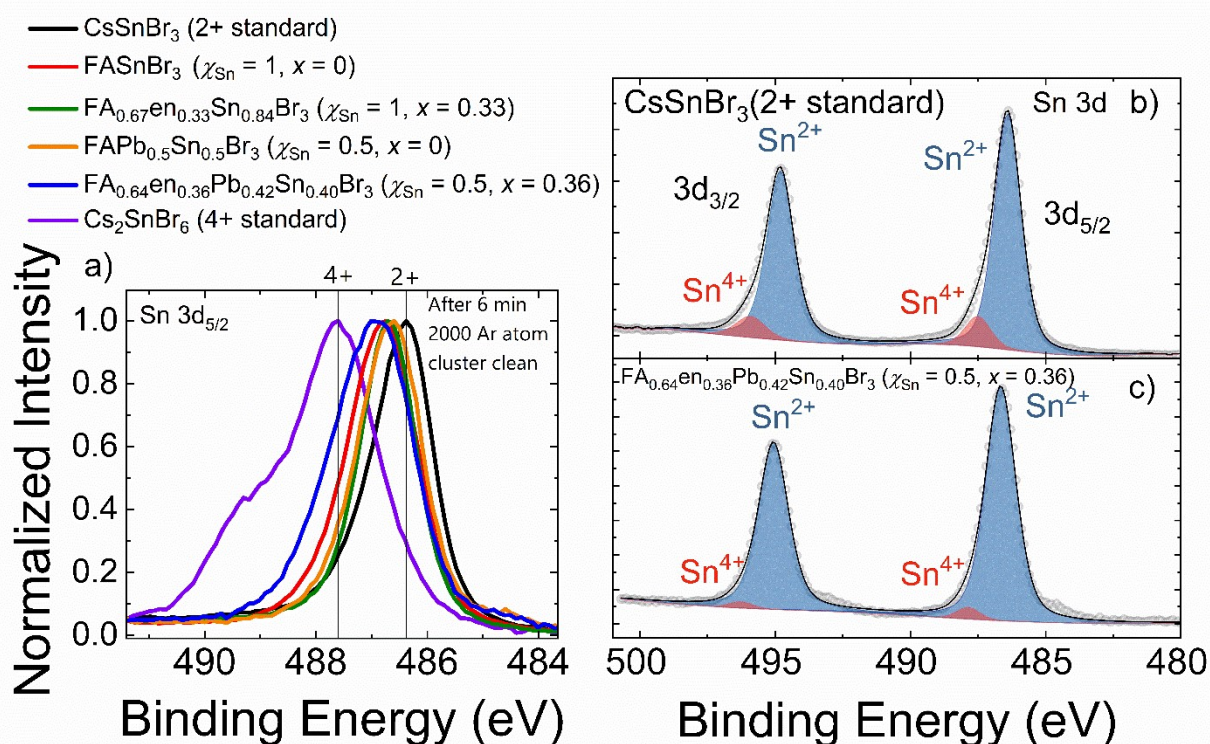
Figure 3. a) Sn 3d 5/2 spectrum of 2 standards (CsSnBr 3 and CsSnBr 6 ) and selected samples. The samples include a hMHP (FA 0.67 en 0.33 Sn 0.84 Br 3 ( \chi_{\text{Sn}} = 1 , x = 0.33 )), a mixed Pb/Sn (FAPb 0.5 Sn 0.5 Br 3 ( \chi_{\text{Sn}} = 0.5 , x = 0 )) and both hMHP and Pb/Sn mixed sample (FA 0.64 en 0.36 Pb 0.42 Sn 0.40 Br 3 ( \chi_{\text{Sn}} = 0.5 , x = 0.36 )). All samples have a similar FWHM and peak position as the FASnBr 3 . All the samples are mainly Sn 2+ with minor Sn 4+ components. b) Fitted Sn 3d spectra for the 2+ standard showing a small (11%) Sn 4+ contribution compared to sample c) FA 0.64 en 0.36 Pb 0.42 Sn 0.40 Br 3 ( \chi_{\text{Sn}} = 0.5 , x = 0.36 ), which showed only 4%.
