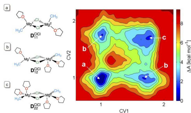
Fig. 5 The free energy map of solvation by THF of (\text{CH}_3)\text{Mg}(\mu\text{-Cl})_2\text{-Mg}(\text{CH}_3) by AIMD and metadynamics. 86 The collective variables (CVs) refer to the coordination number of THF to the two Mg's, according to eqn (1). Panels (a–c) indicate the structures corresponding to the free energy basins. Figure adapted from ref. 82, under ACS AuthorChoice agreement.
